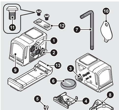
Fig. 1 Overview including A-CUT™ Mount plate - Micro™ conversion kit*
