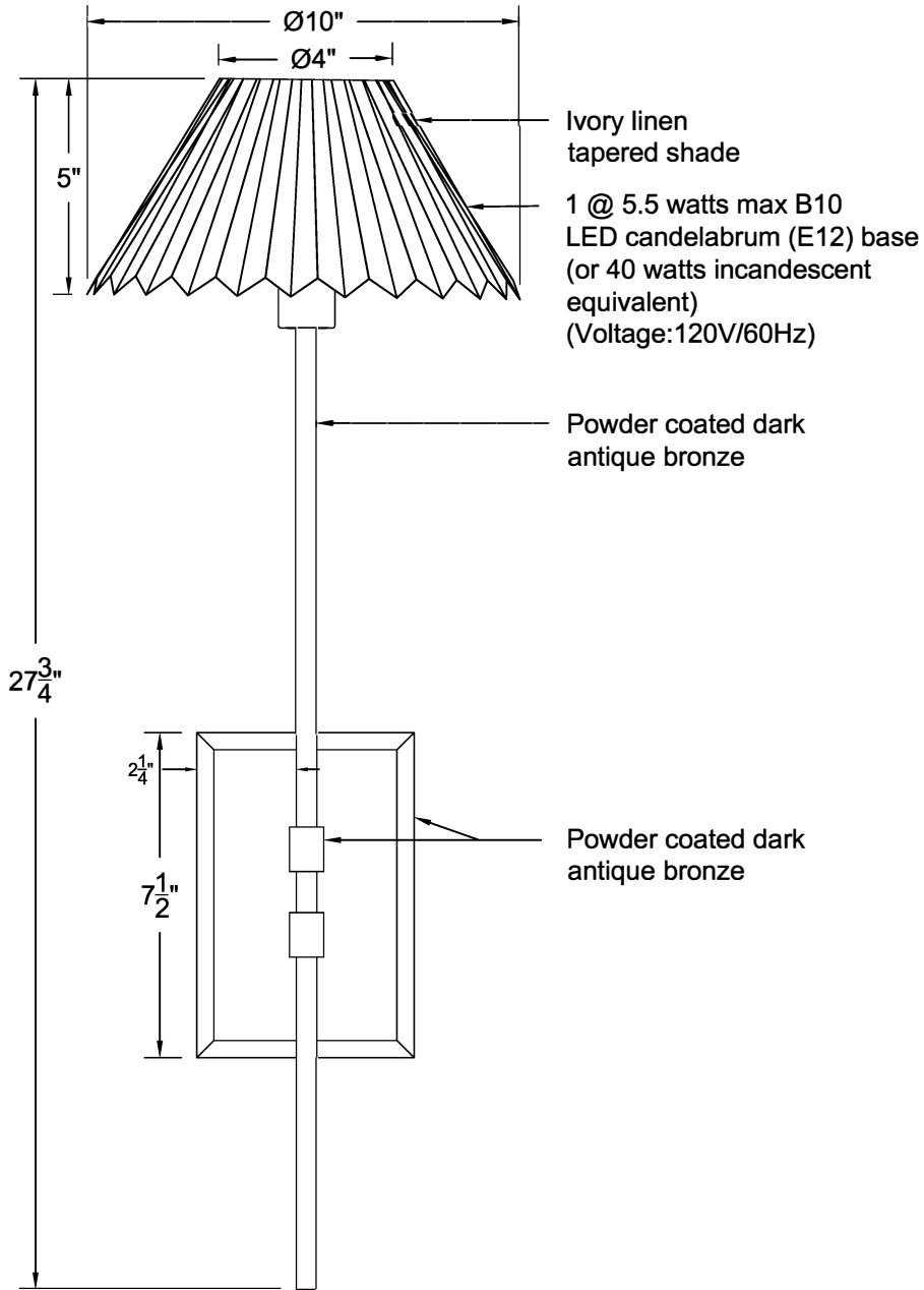
FRONT VIEW
