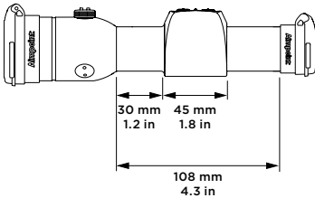
Aimpoint® Hunter™ series H34S and H30S
