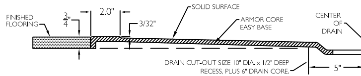
CROSS SECTION OF THRESHOLD
