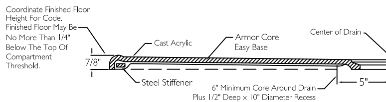
CROSS SECTION OF THRESHOLD
