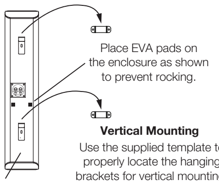
Fig. 4 Wall Mounting
