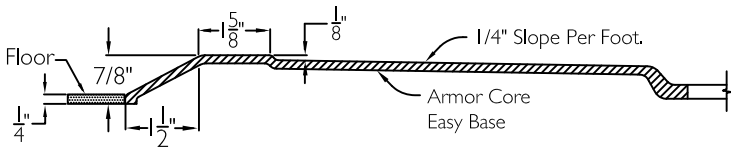
CROSS SECTION OF THRESHOLD
