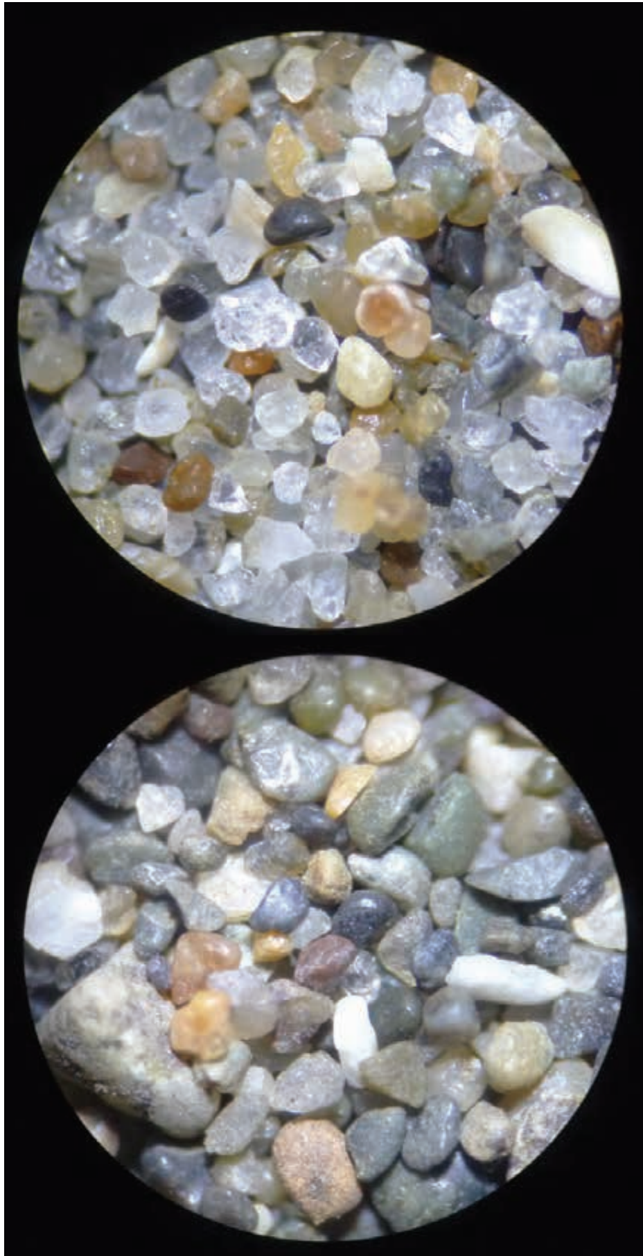
Sand from two different California beaches 40x
