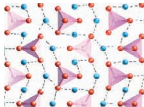
The tetrahedrons are shown in pink with red oxygens at the points. The blue balls represent metal atoms, perhaps Fe or Mg. The dashed lines represent electrical attraction keeping the atoms in place.
