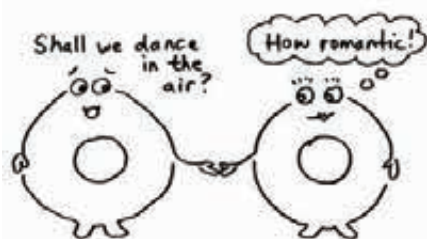
O 2 is a molecule.
