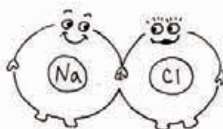
NaCl is both a molecule and a compound.
