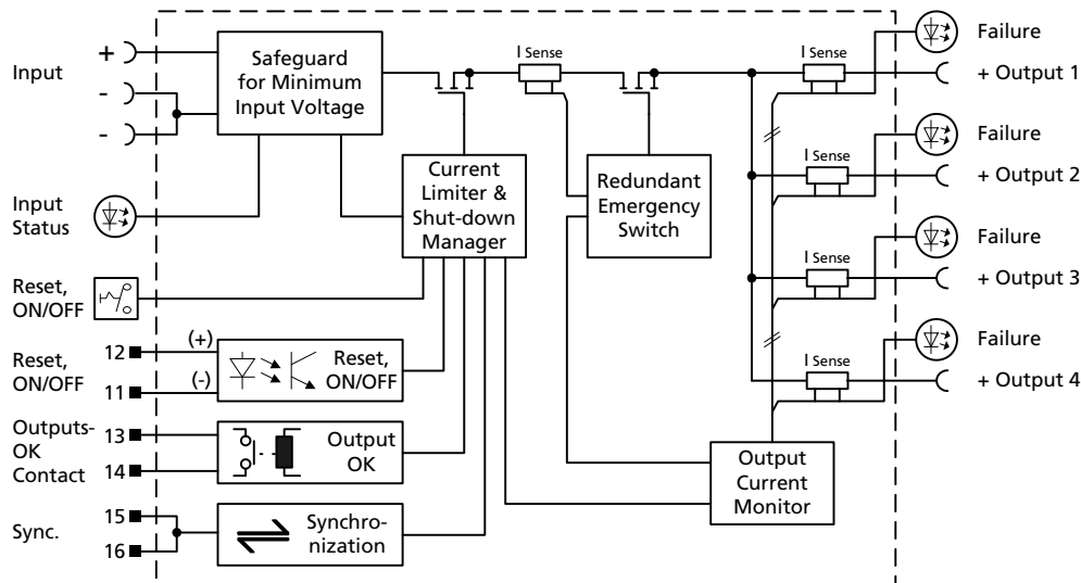
Fig. 11-1 Functional diagram
