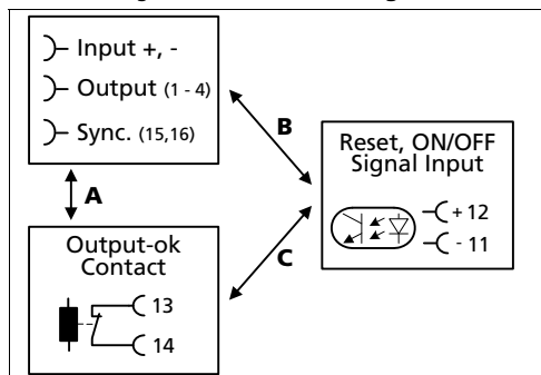
Fig. 22-1 Dielectric strength
