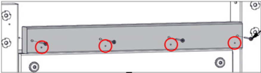
391 (x4) SCREW - 2"
