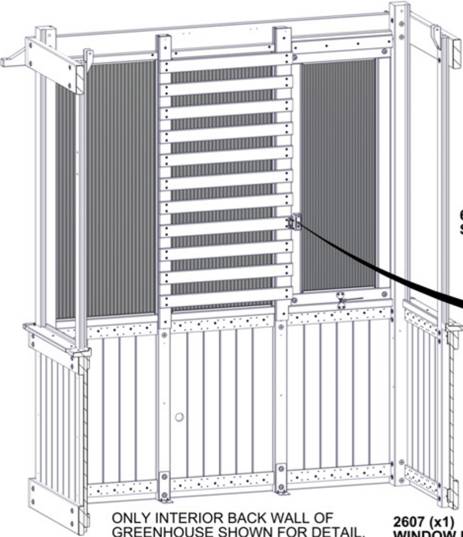
627 (x2) SCREW - 3/4"
