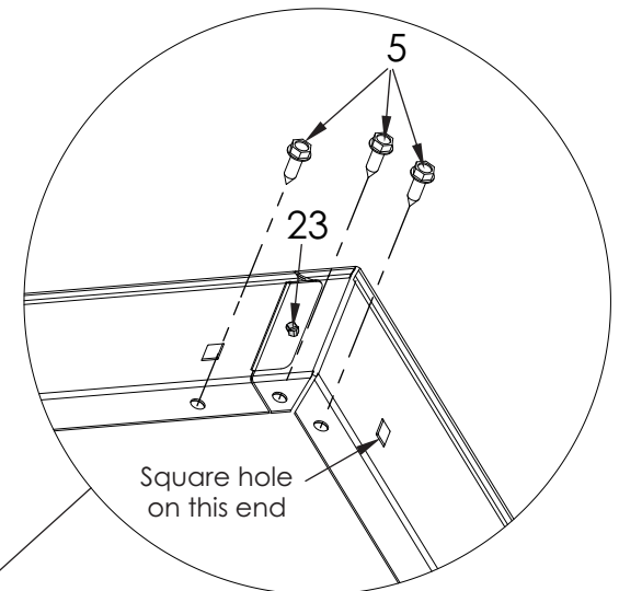
Detail F
