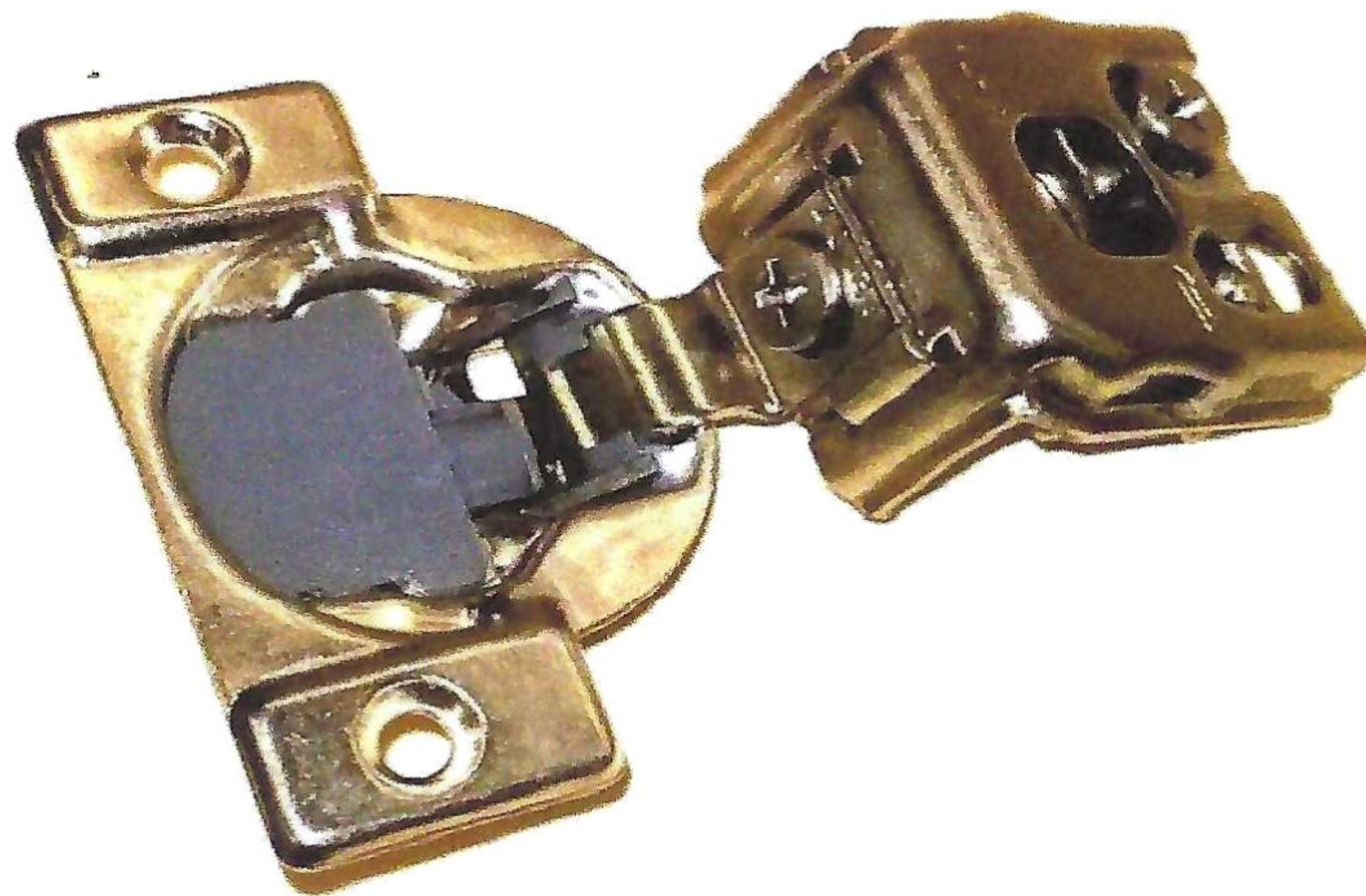
HINGE P/N 9394-000
