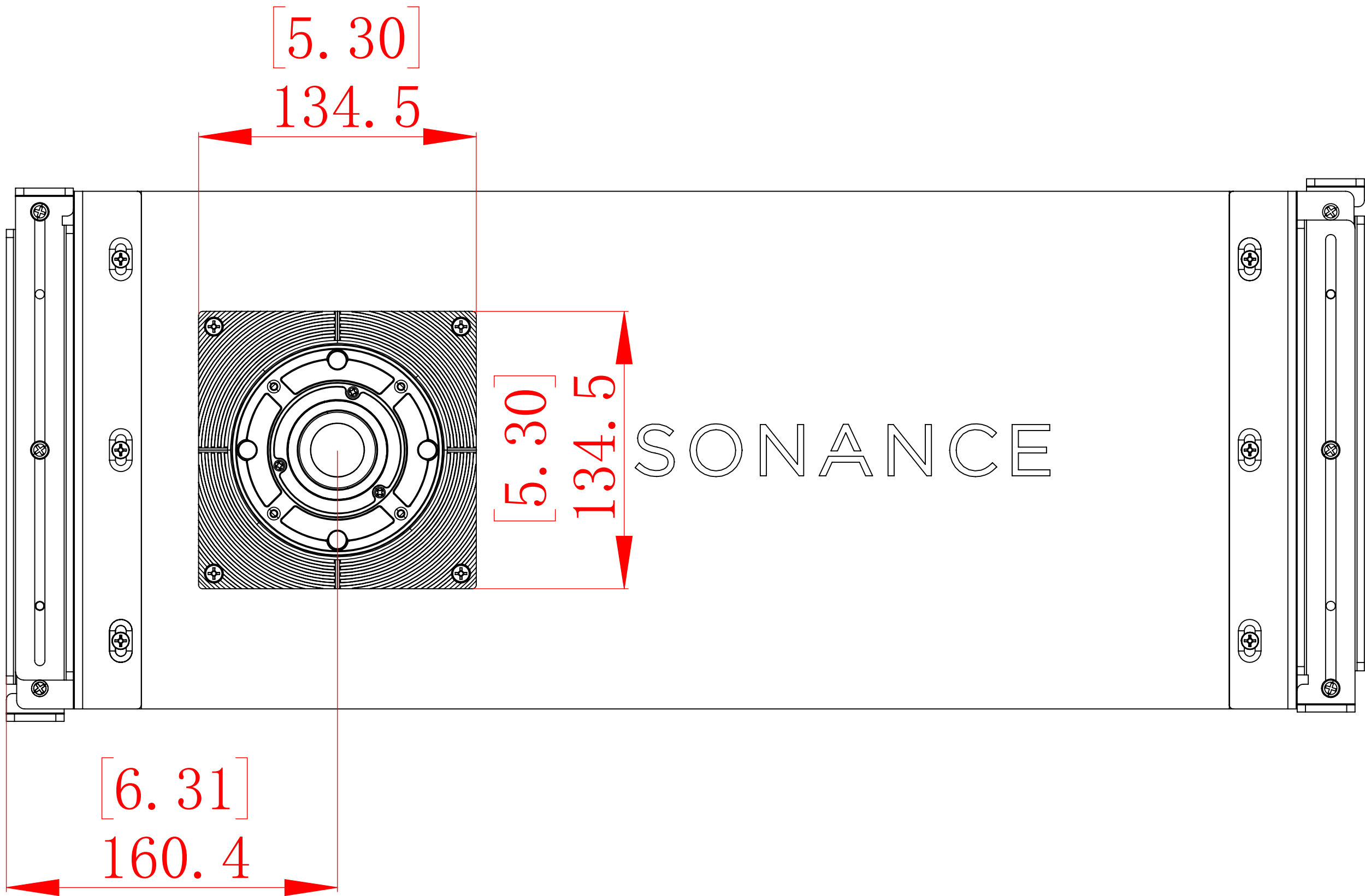
FRONT VIEW
