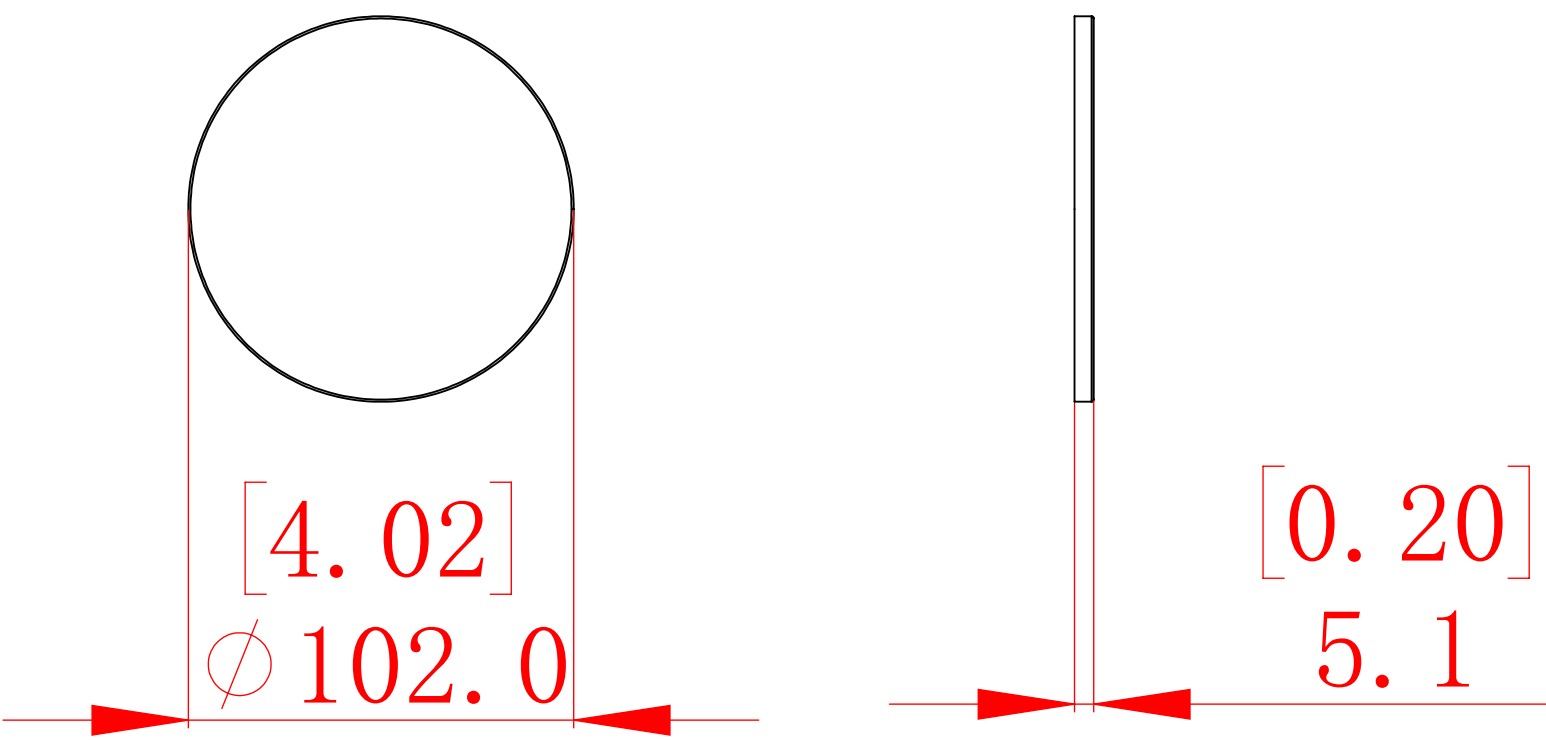
SIDE VIEW
