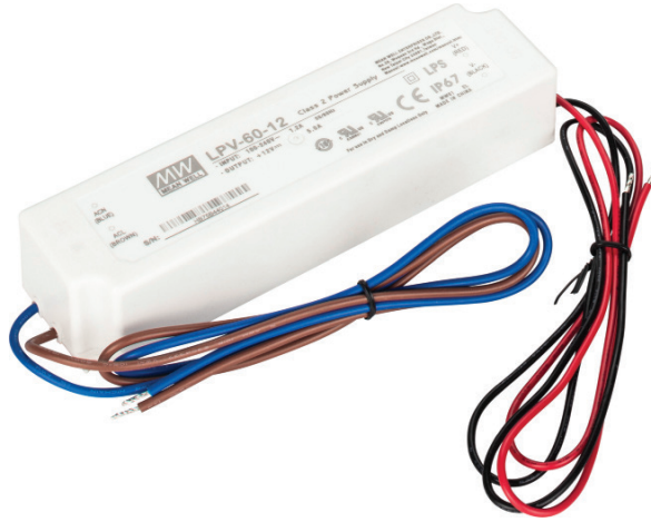
T-24-60W-WP-HW
