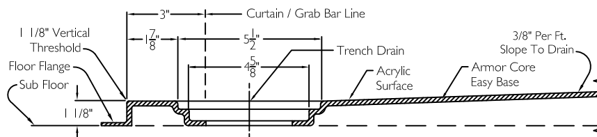
CROSS SECTION OF SHOWER BASE
