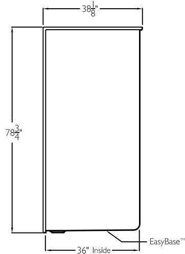
CROSS SECTION OF SHOWER BASE
