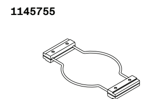
1145755 COLANDER HOLDER DETAILS 16-1/4" x 5-1/2"
