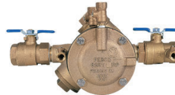
Febco 825Y Reduced Pressure
