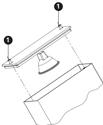
Drawing 2 - Relamping
