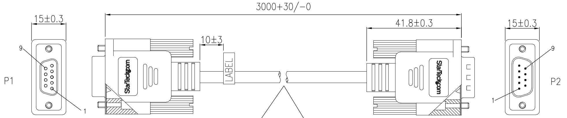
MATING VIEW
