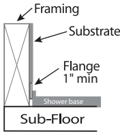
Flange Details: (U.S.)
