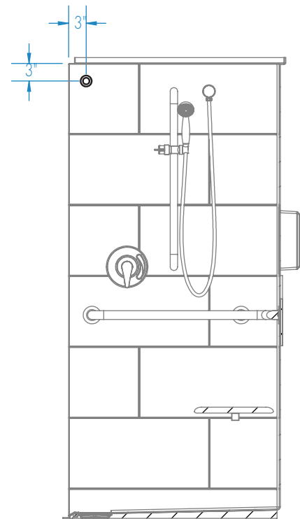
SECTION C-C
