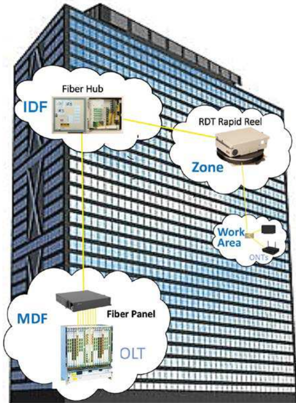
Figure 2: Hub and terminal architecture
