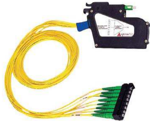
Figure 7: Plug-and-play splitter
