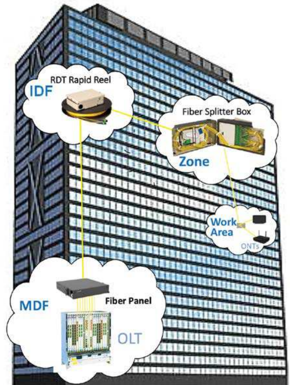
Figure 3: Distributed splitter architecture
