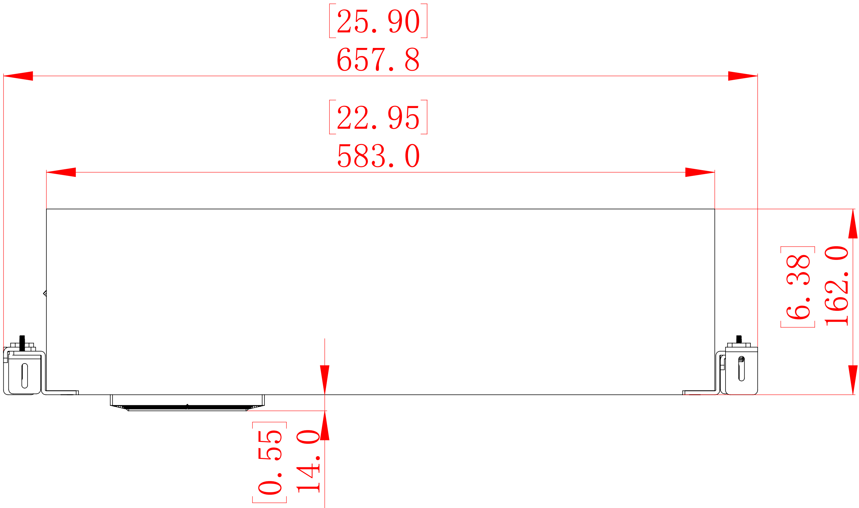
SIDE VIEW
