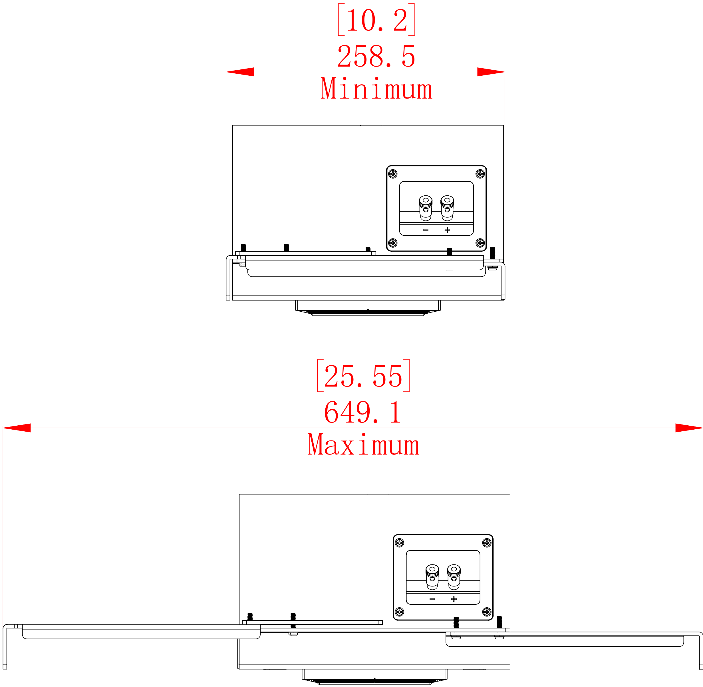
SIDE VIEW
