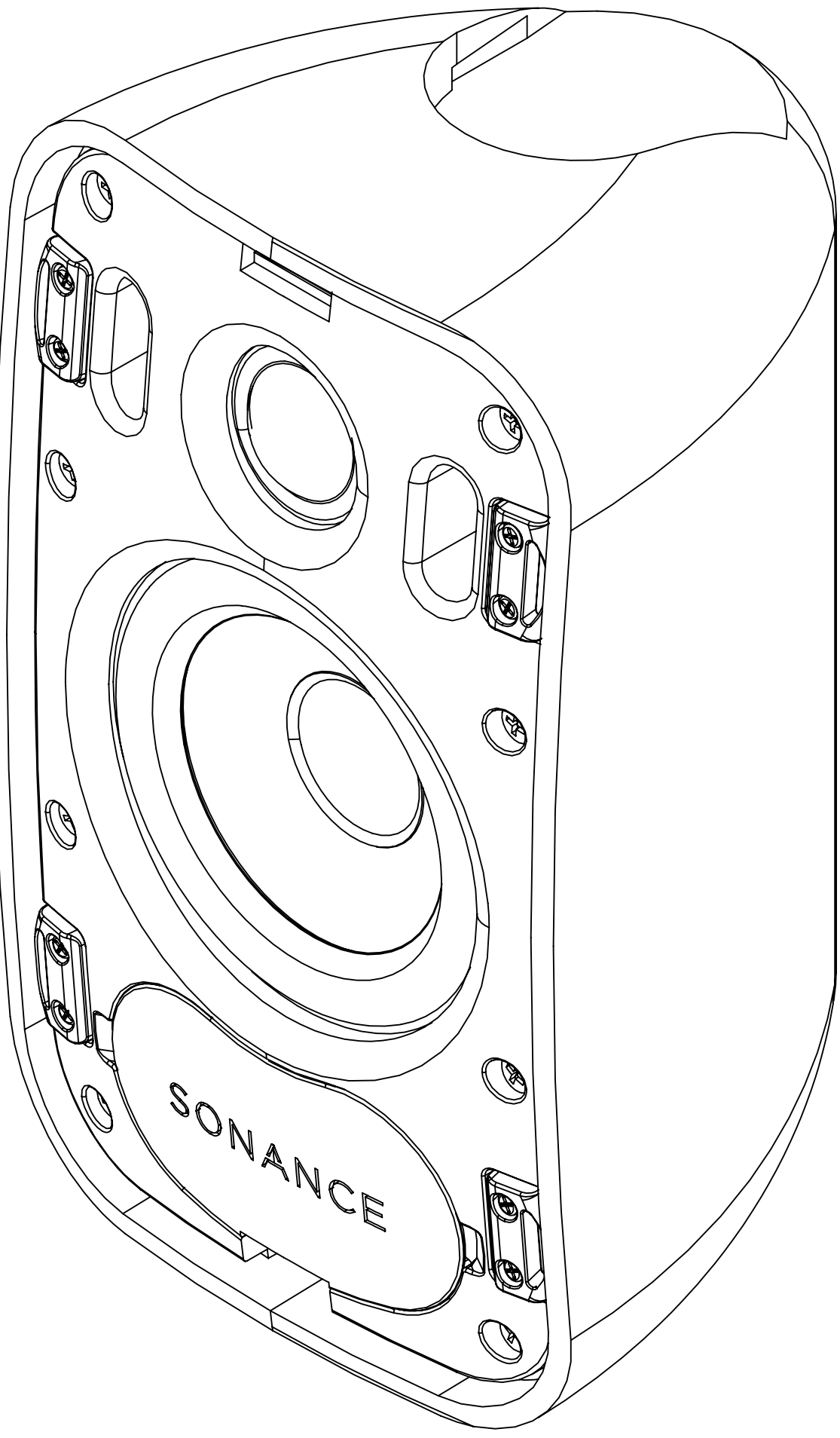
ISOMETRIC
