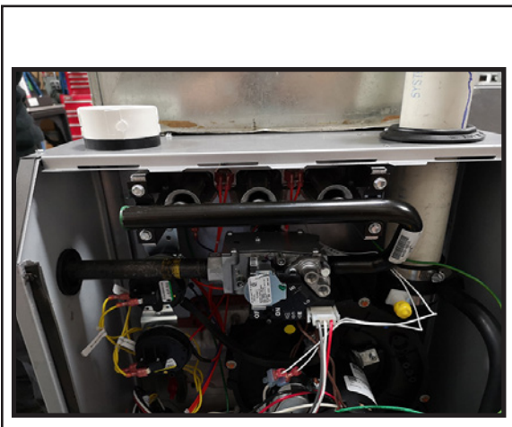
FIGURE 24 - INSHOT BURNER ASSEMBLY
