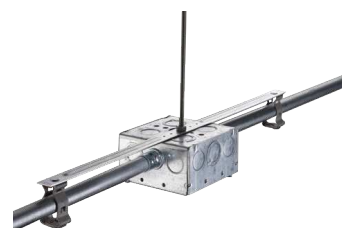
CEILING BRACKETS
