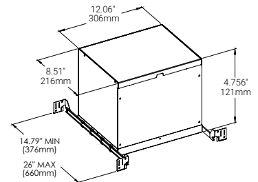
AT/IC BOX 47138-018 (Trim/Trimless)
