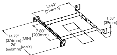
NEW CONSTRUCTION PLATE 47135-017 (Trim/Trimless)
