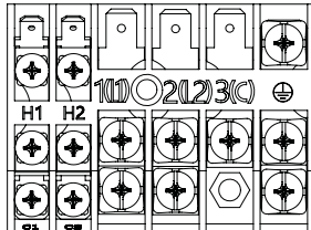
Outdoor Unit Terminal Block for 230V Models
