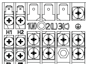
Outdoor Unit Terminal Block for 115V Models
