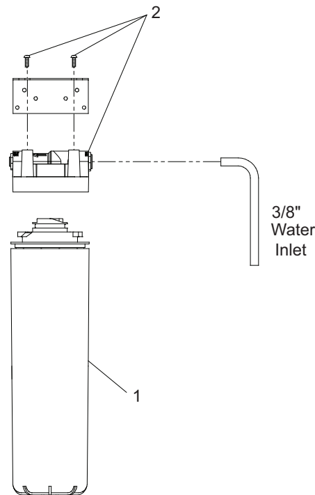
WATER FILTER EXPLODED VIEW
