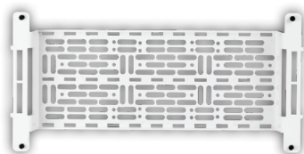
Mounting plate with 1.5" of elevation allows for 2 nd layer of mounting. Plate included with -V1 models. Plate part number: AC1050
