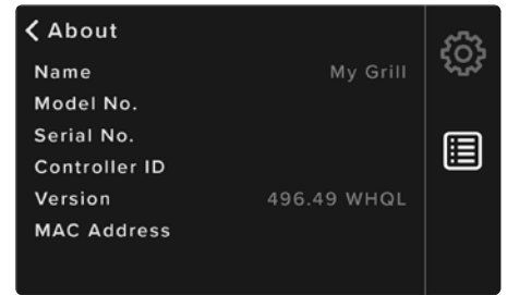
FIGURE 6: ABOUT SCREEN
