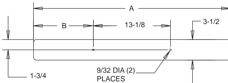
REF.NO. 3 (FOR 10P) A = 33-1/2 B = 10-3/16 REF.NO. 7 (FOR 17P) A = 39 B = 12-15/16 1 X 4 PRESSURE TREATED WOOD
