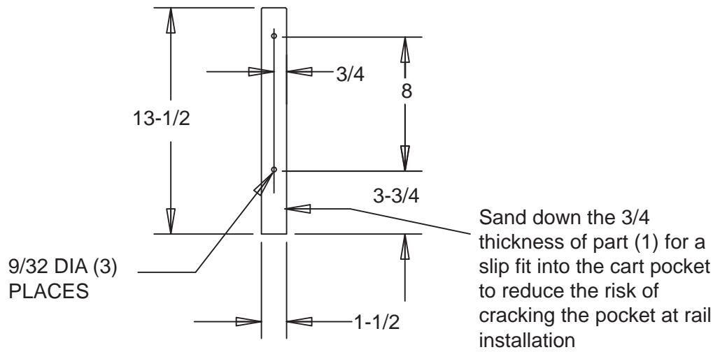
REF.NO. 1 (FOR 10P AND 17P) 1 X 2 PRESSURE TREATED WOOD
