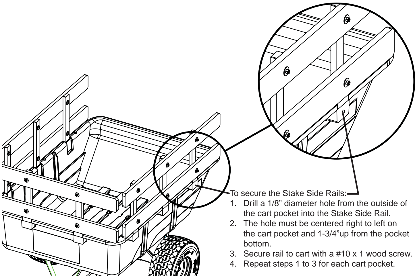
Fig 4 - Permanently Secure Sides
