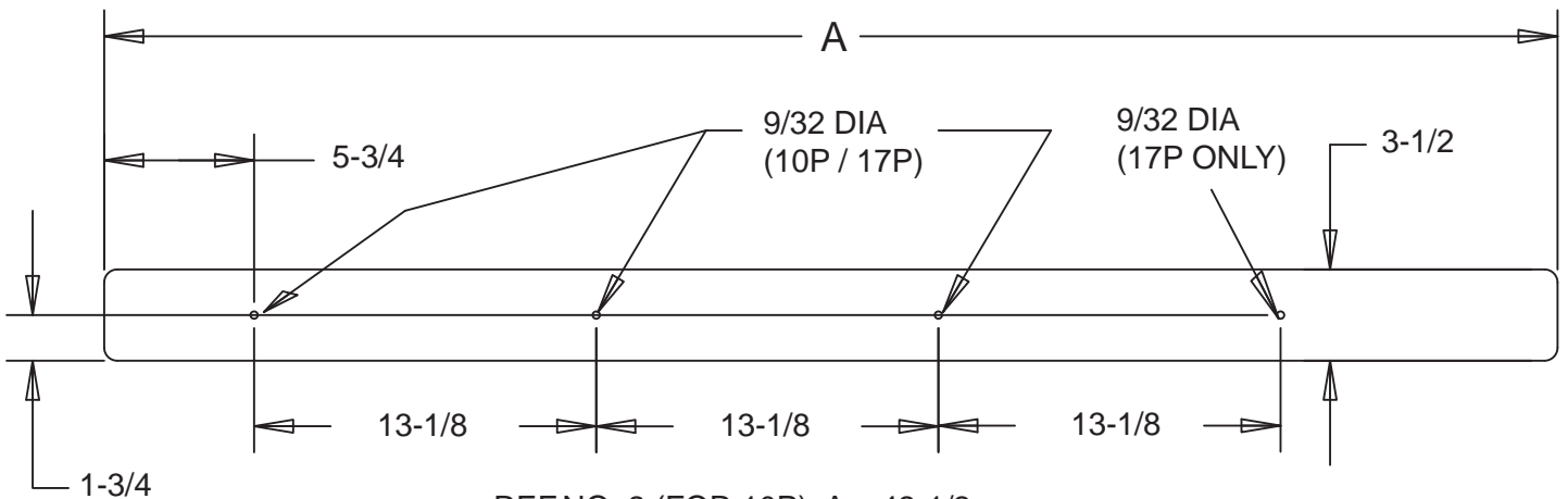
REF.NO. 2 (FOR 10P) A = 42-1/2 REF.NO. 8 (FOR 17P) A = 55-3/4 1 X 4 PRESSURE TREATED WOOD
