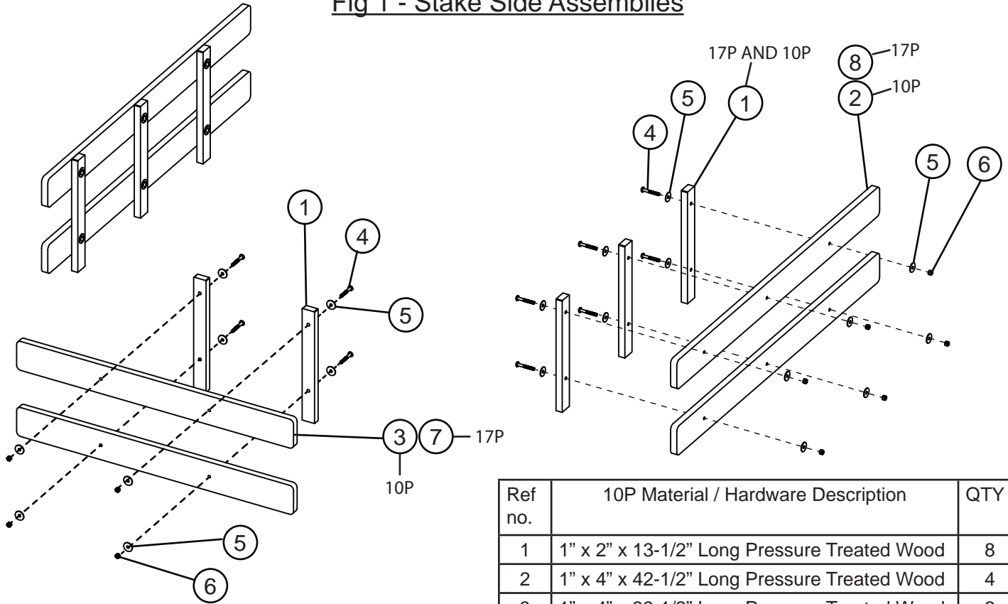
Fig 1 - Stake Side Assemblies
