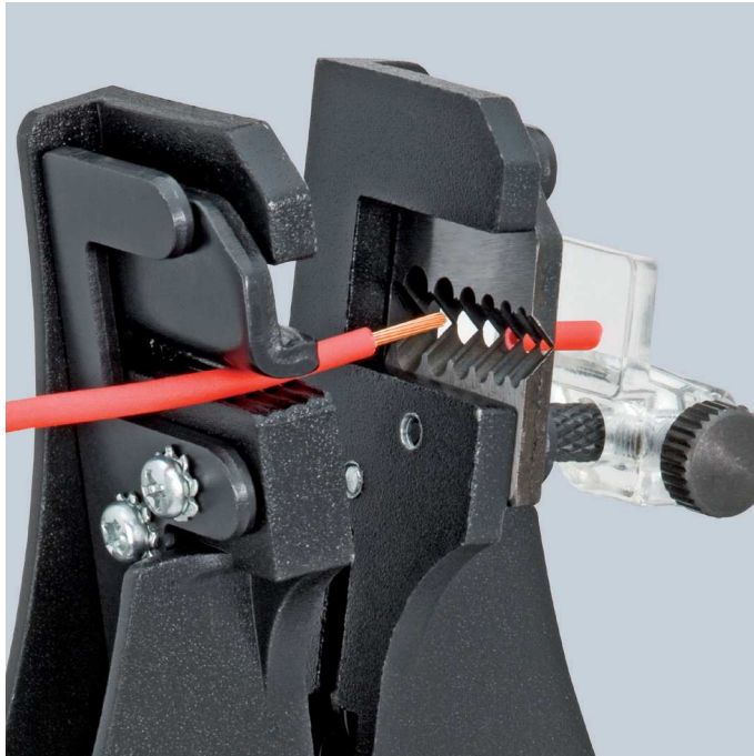
Adjustable length stop for repetitive work
