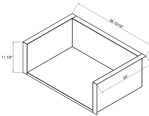
MODEL# XOG36JACKET 36" SS Insulated Sleeve
