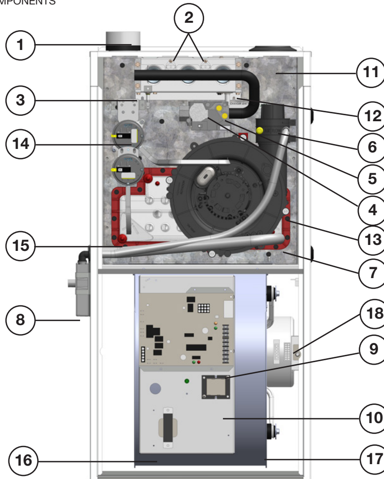
FIGURE 1 - FURNACE COMPONENTS
