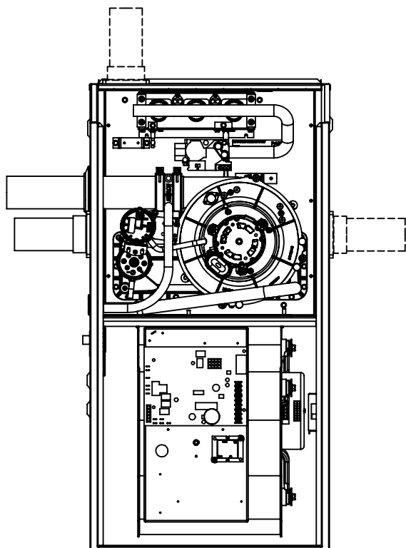
LEFT VENT - LEFT DRAIN INSTALLATION (INTERNAL)
