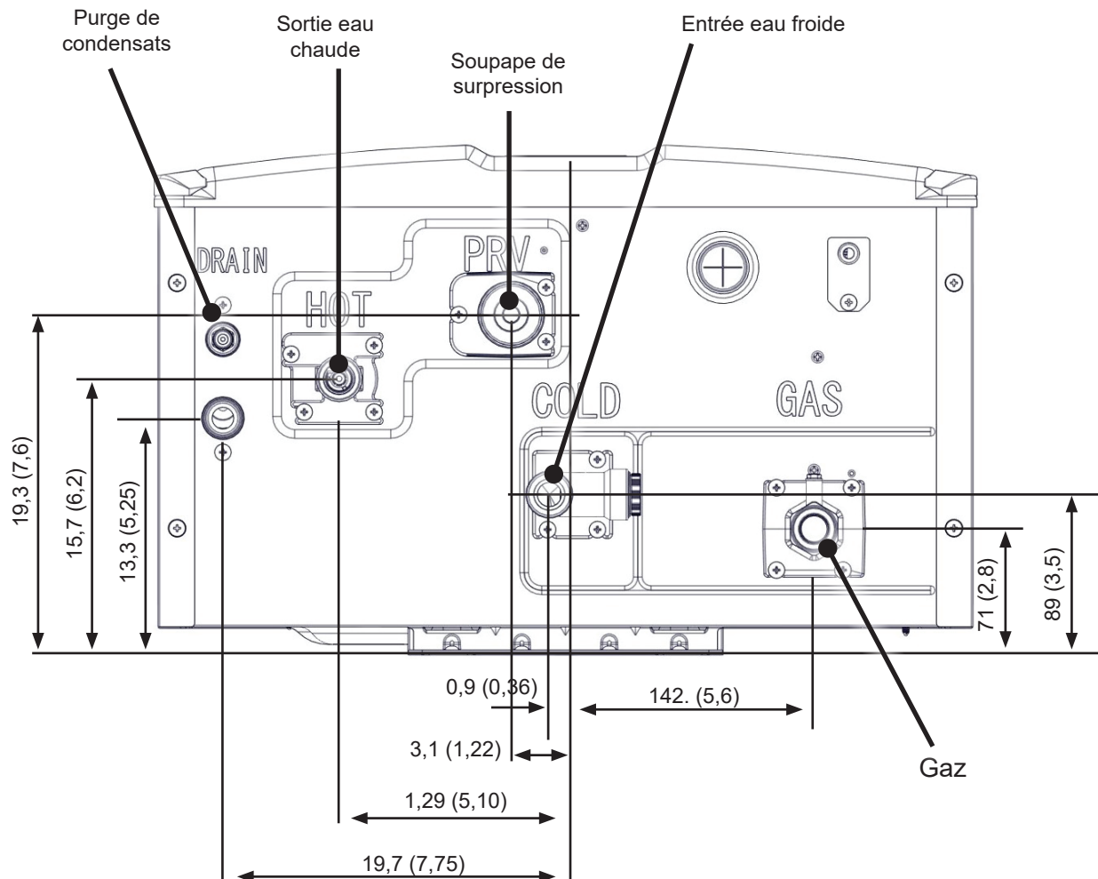
Figure 6: Raccords d'alimentation
