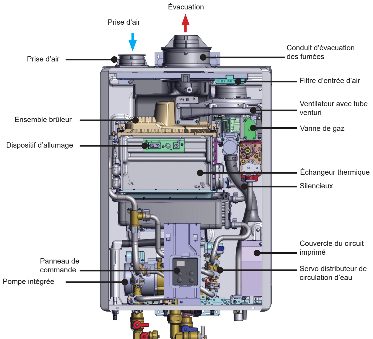
Figure 3: Composants
