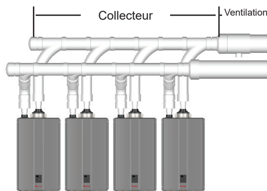
Figure 50: Installation de circuit commun d'évacuation PVC/CPVC
