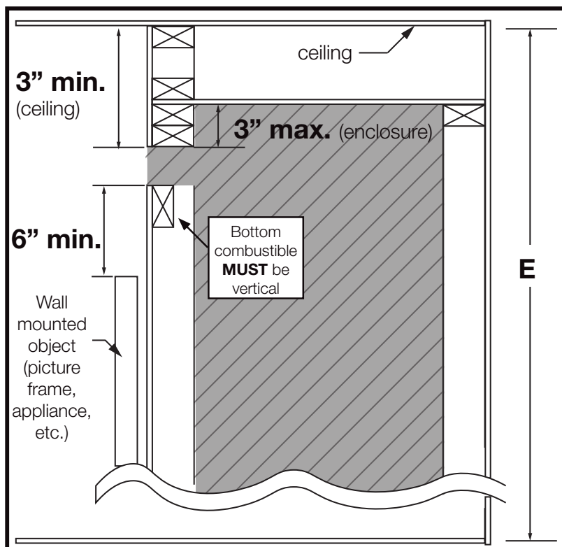
SIDE VIEW
