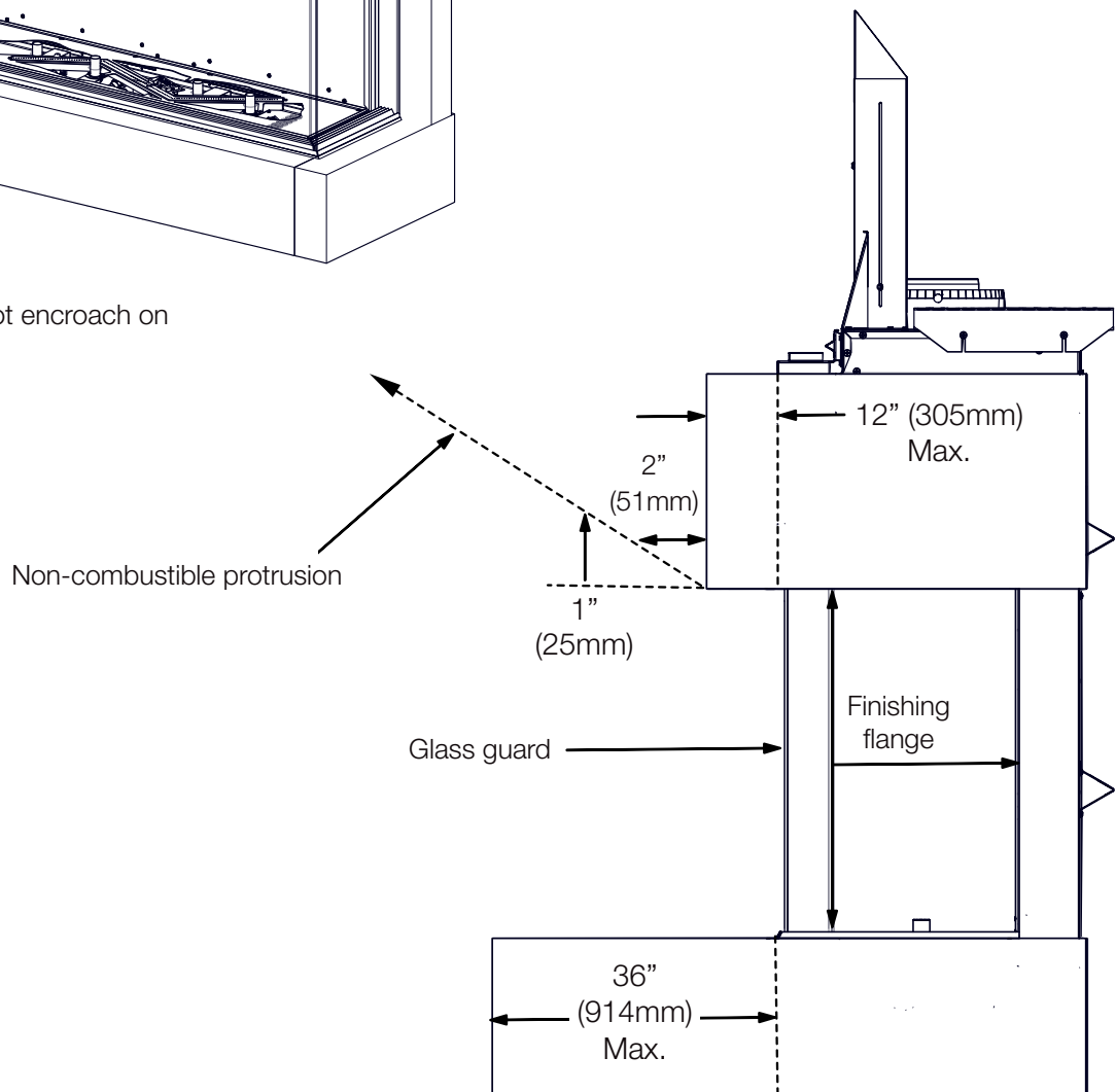
Side View
