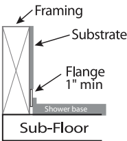
Flange Details: (U.S.)
