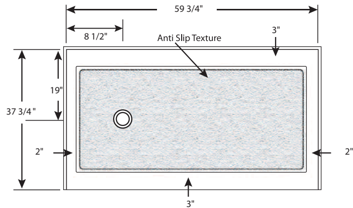
Top View – Left Drain
