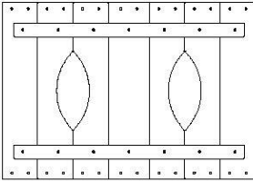
WP13 | PANEL DE LA PARED - W2A01477 (x2) | 1 1/4"x16 5/8"x24 1/4" (32x430x616)
