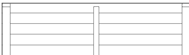
RP1 | PANEL SUPERIOR DEL TECHO - W2A01478 (x2) | 1 3/8"x15 7/8"x56 1/4" (35x404x1428)
