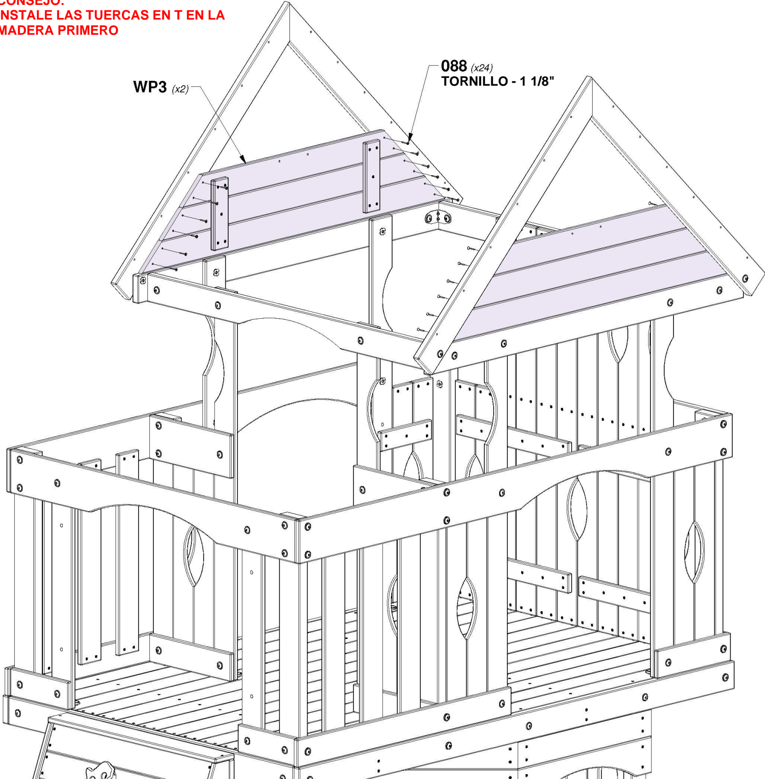
WP3 GABLETE - W2A01476 (x2) 1 1/4"x10 1/8"x50 3/8" (32x258x1280)
