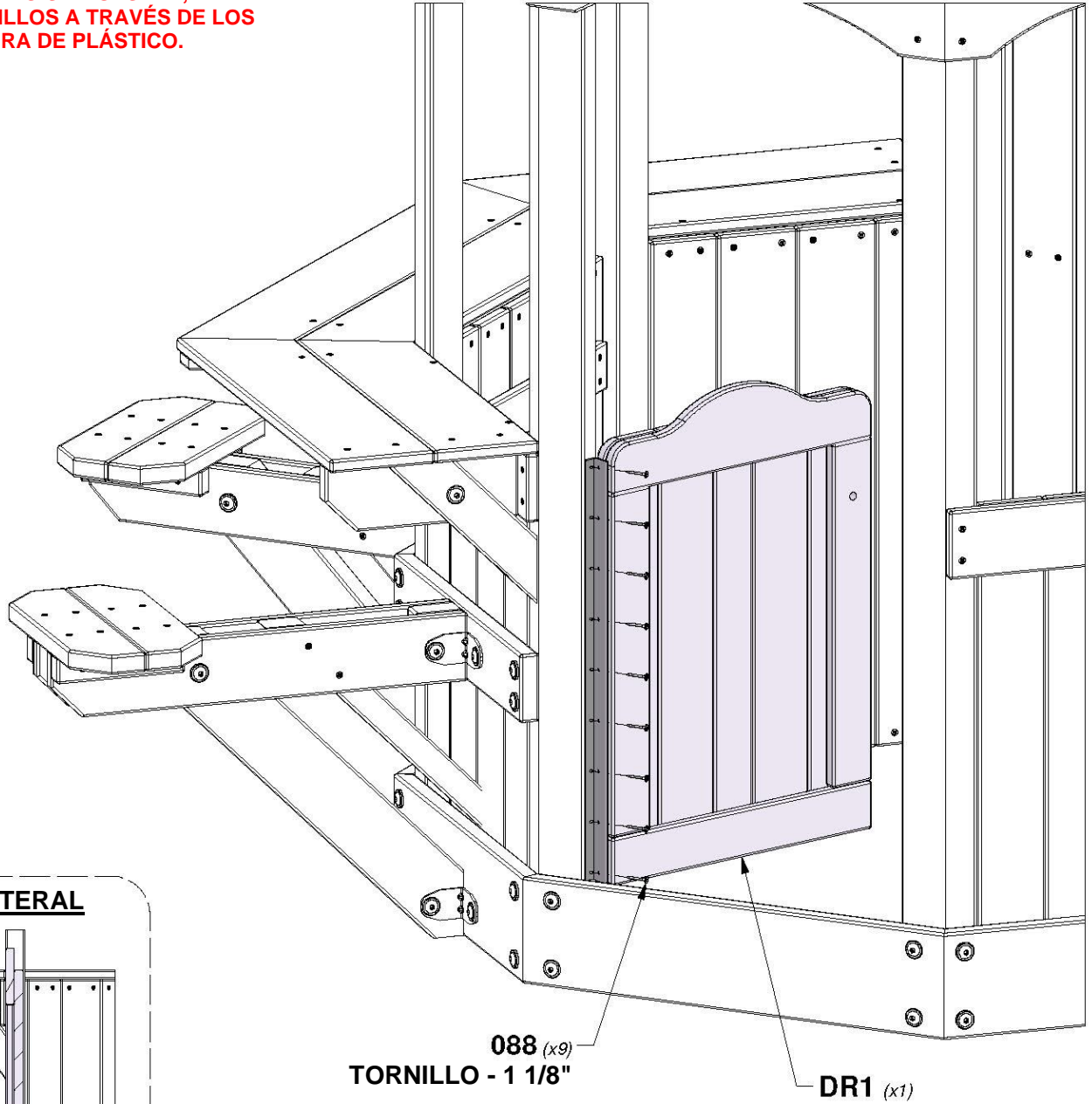
DR1 | PANEL DE LA PUERTA - W2A01482 (x1) | 1 1/4"x16"x23 1/2" (32x406x596)
