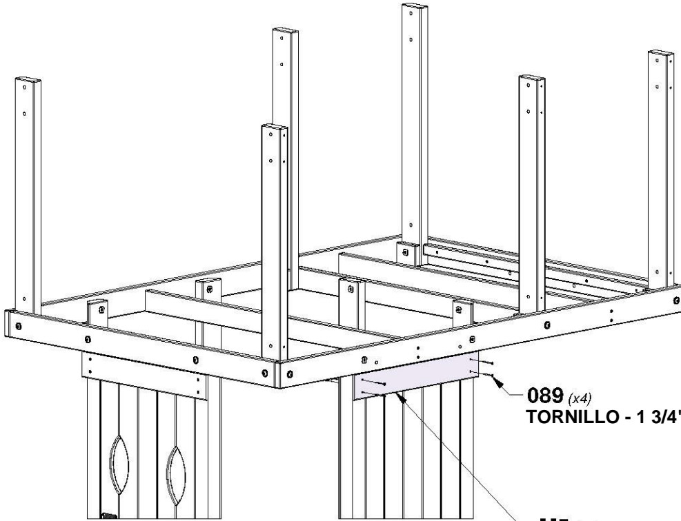
M5 | GUÍA DE PARED - W4L04465 (x1) | 5/8"x3 3/8"x22" (16x86x563)
