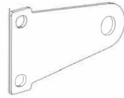
B03 SUPPORT DE LOQUET - A4M02413 (x2) 1/8"x2 3/16"x4 1/8" (2.5x56x104)
