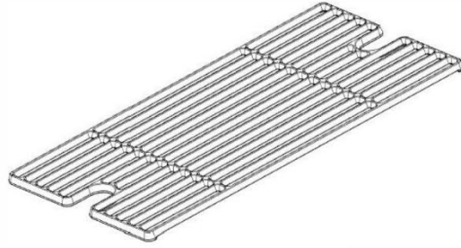
G02 GRILLE -A4M02145 (x3) 7/16"x10 1/2"x20 1/2" (12x266x520)
