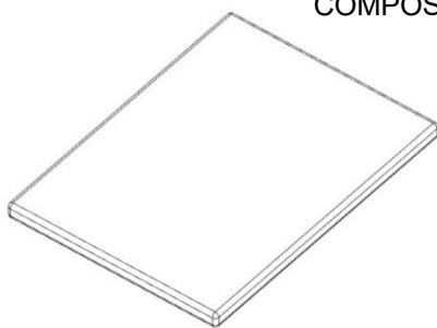
T01 PLATEAU DE TABLE-W4L18241 (x2) 1 1/4"x17 11/16"x23 5/8" (32x450x600)
