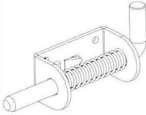
DL01 LOQUET DE PORTE - A4M02496 (x4) 1 5/16"x1 7/8"x4 3/8" (33x47x111)
