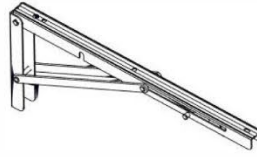
2094 SUPPORT DE TABLE -A4M02094 (x4) 1 3/8"x6 13/16"x15 15/16" (34x173x405)
