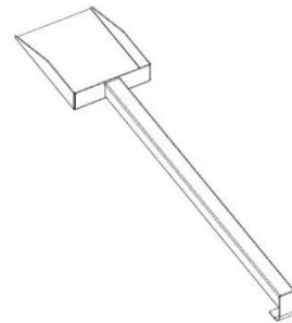
SH01 PELLE - A4M02513 (x1) 2 1/4"x4 7/8"x31 7/16" (57x124x798)
