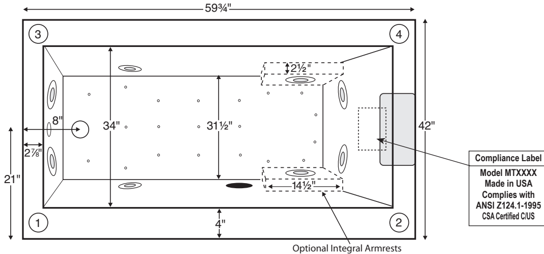
Optional Integral Armrests
