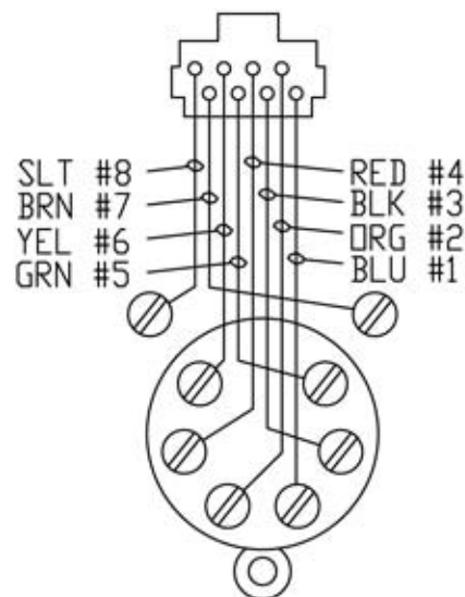
WIRE CONNECTIONS REAR VIEW (TYP)
