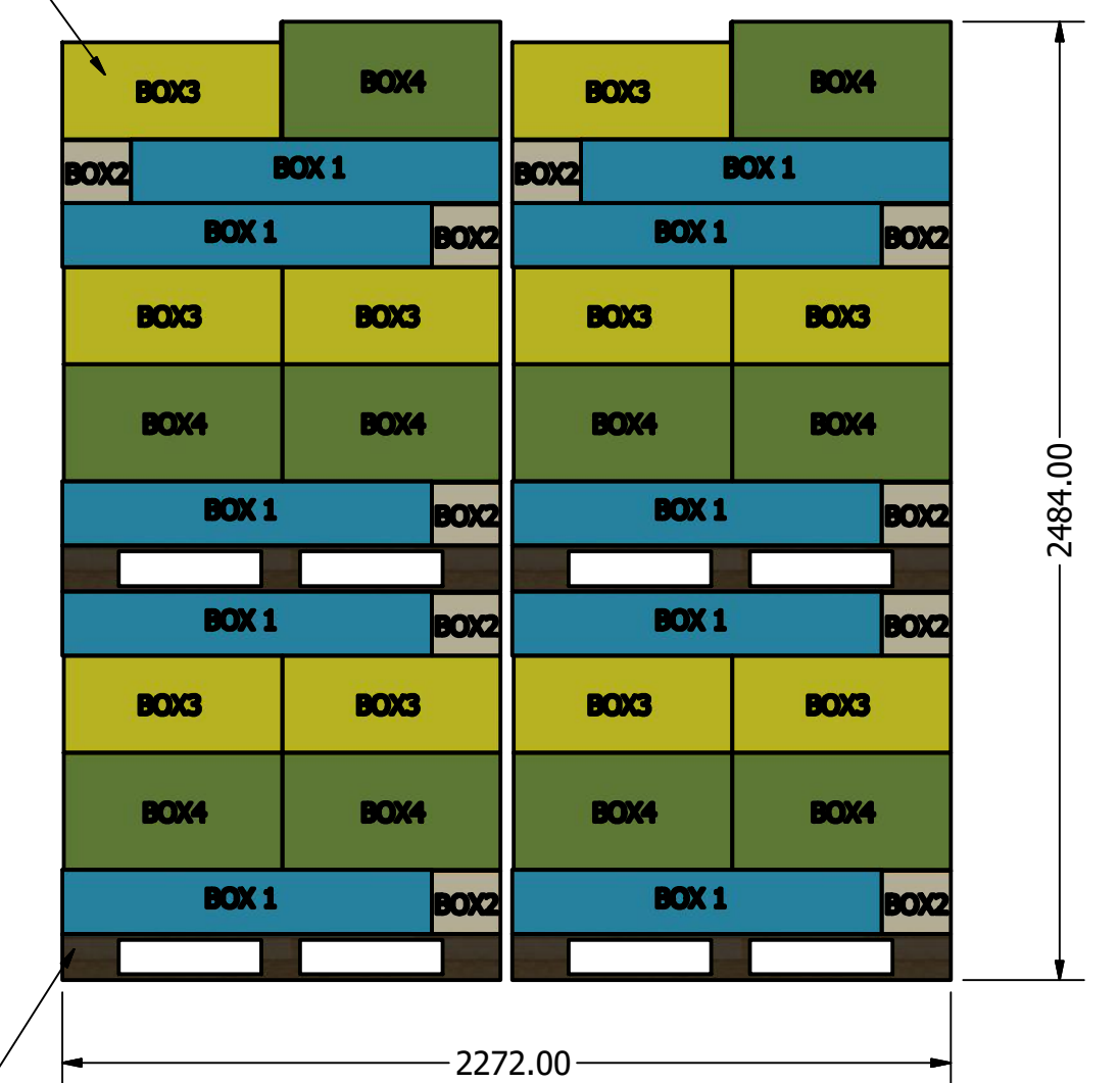
End view
