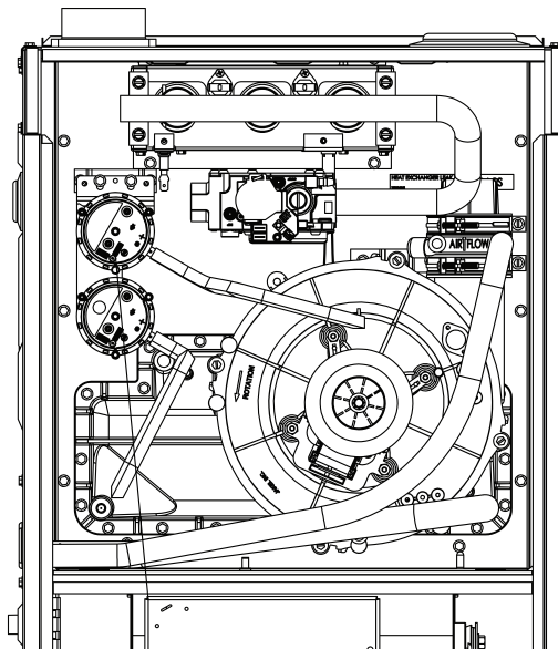
TOP VENT - LEFT DRAIN INSTALLATION (INTERNAL)
