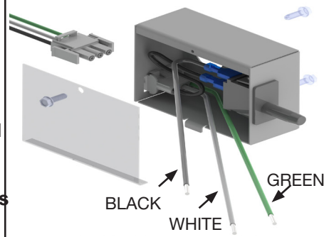
FIGURE 31 - ELECTRICAL CONNECTIONS / MOLEX CONNECTOR
