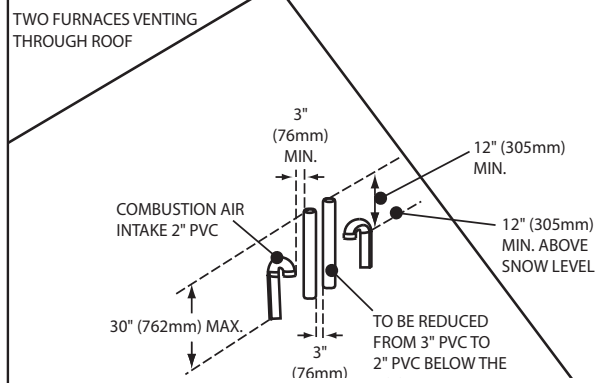
FIGURE 13 - MULTIPLE VENTING (STANDARD VERTICAL)
