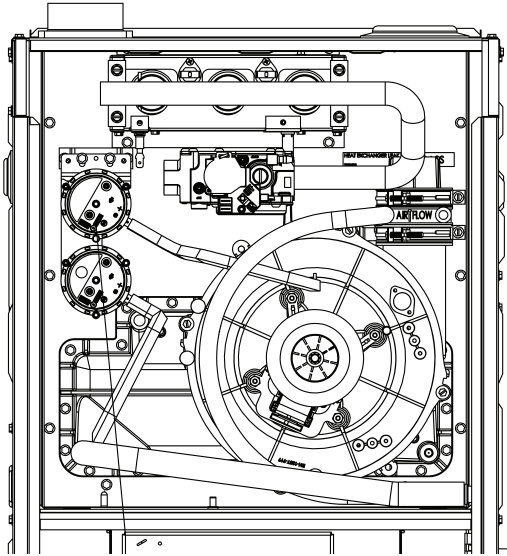
TOP VENT - RIGHT DRAIN INSTALLATION (INTERNAL)
