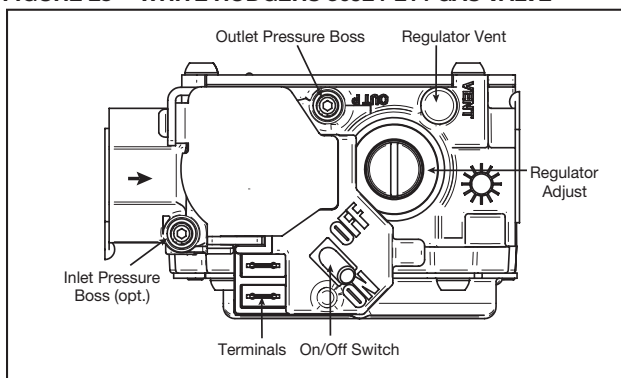
FIGURE 28 - WHITE RODGERS 36J24-214 GAS VALVE
