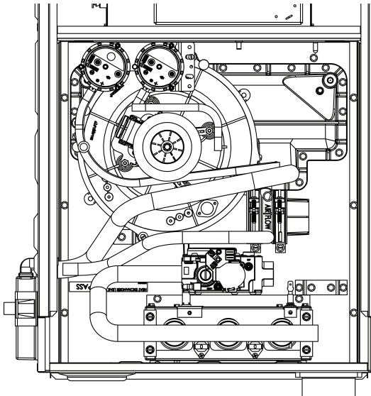
FIGURE 19 - DOWNFLOW VENT AND DRAINING OPTION
