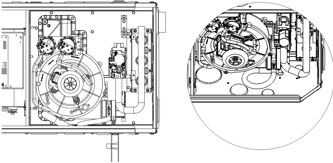
FIGURE 18 - HORIZONTAL RIGHT VENT AND DRAINING OPTION CONTINUED
