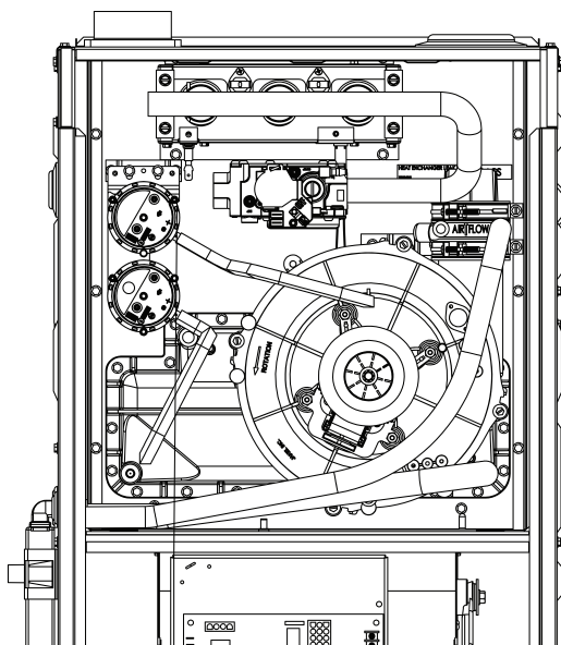
TOP VENT - LEFT DRAIN INSTALLATION (EXTERNAL)
