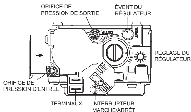
FIGURE 28 - SOUPAPE DE GAZ WHITE RODGERS 36J24-214
