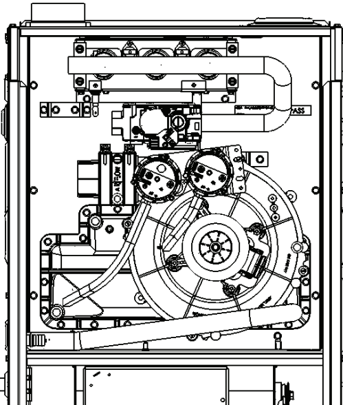
LEFT VENT - LEFT DRAIN INSTALLATION (INTERNAL)
