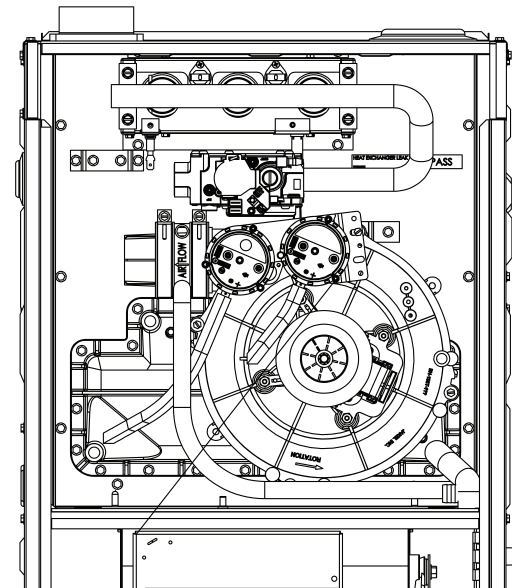
LEFT VENT - RIGHT DRAIN INSTALLATION (INTERNAL)
