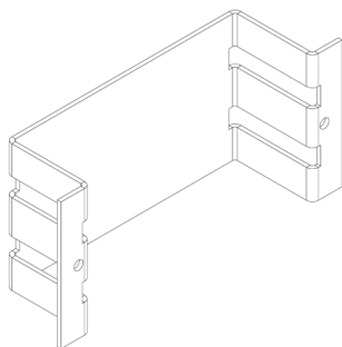
FIGURE 3 - INTERNAL TRAP BRACKET
