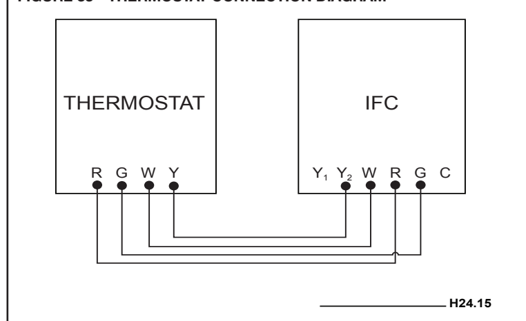
FIGURE 33 - THERMOSTAT CONNECTION DIAGRAM
