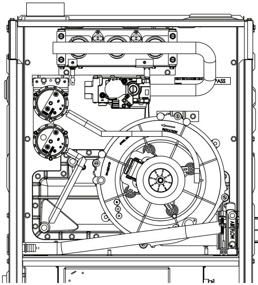
FIGURE 16 - UPFLOW VENT AND DRAINING OPTION CONTINUED
