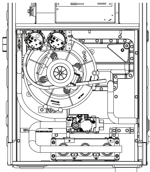
RIGHT VENT INSTALLATION - LEFT DRAIN (INTERNAL)
