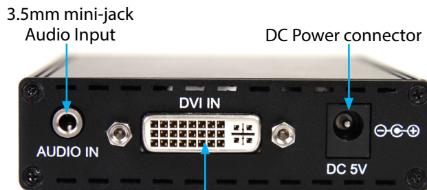
3.5mm mini-jack Audio Input DC Power connector DVI connector (input)
