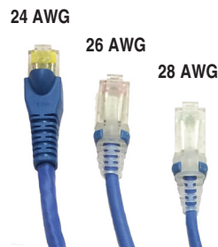
Construction: Smaller 28 AWG construction results in a smaller bend radius for easier routing in tight spaces.
