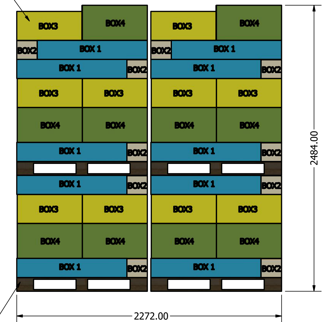
End view
