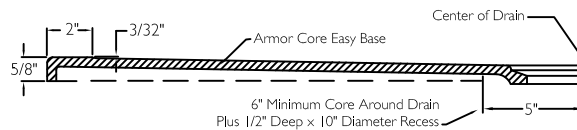
CROSS SECTION OF THRESHOLD.
