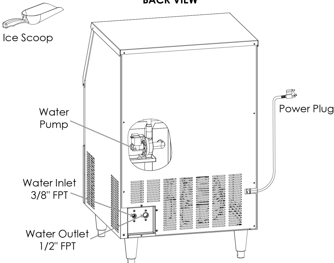
BACK VIEW
