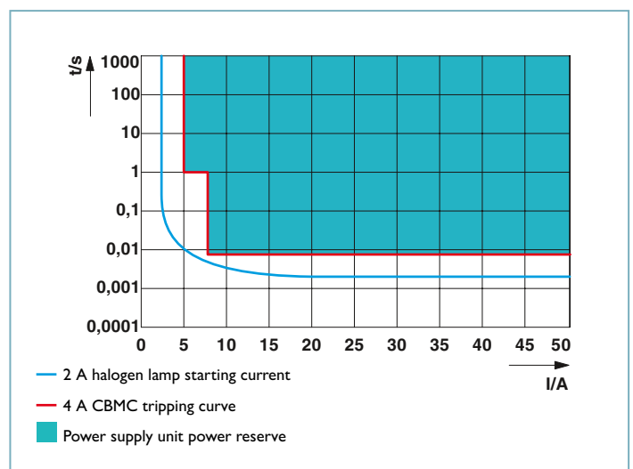
Fig. 24: Thanks to intelligent short-circuit and starting current detection, electronic circuit breakers can shut down more accurately under identical conditions. This means that a much smaller reserve is needed than with comparable thermomagnetic device circuit breakers (cf. Fig. 23).
