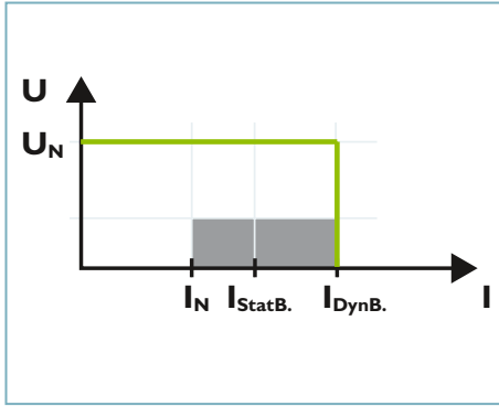
Fig. 2: Power Supply U/I characteristic curve
